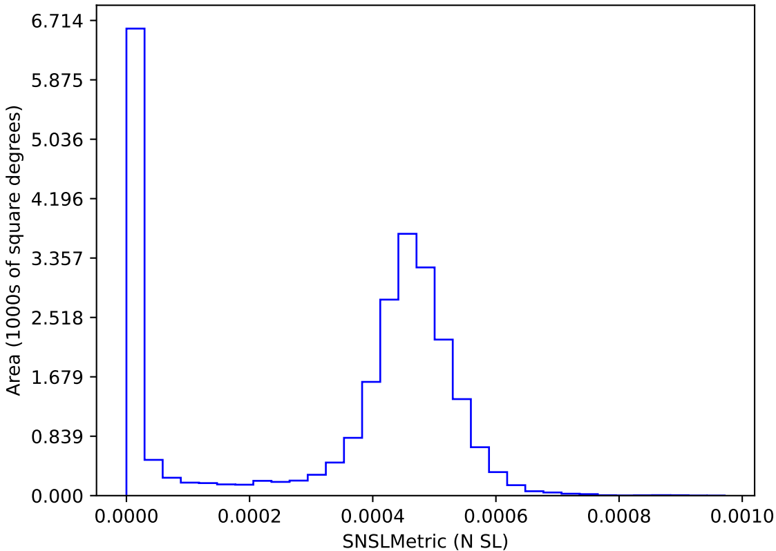
too_elab_2yr_r128_d2_ugrizy_v3.4_10yrs : SNSLMetric
