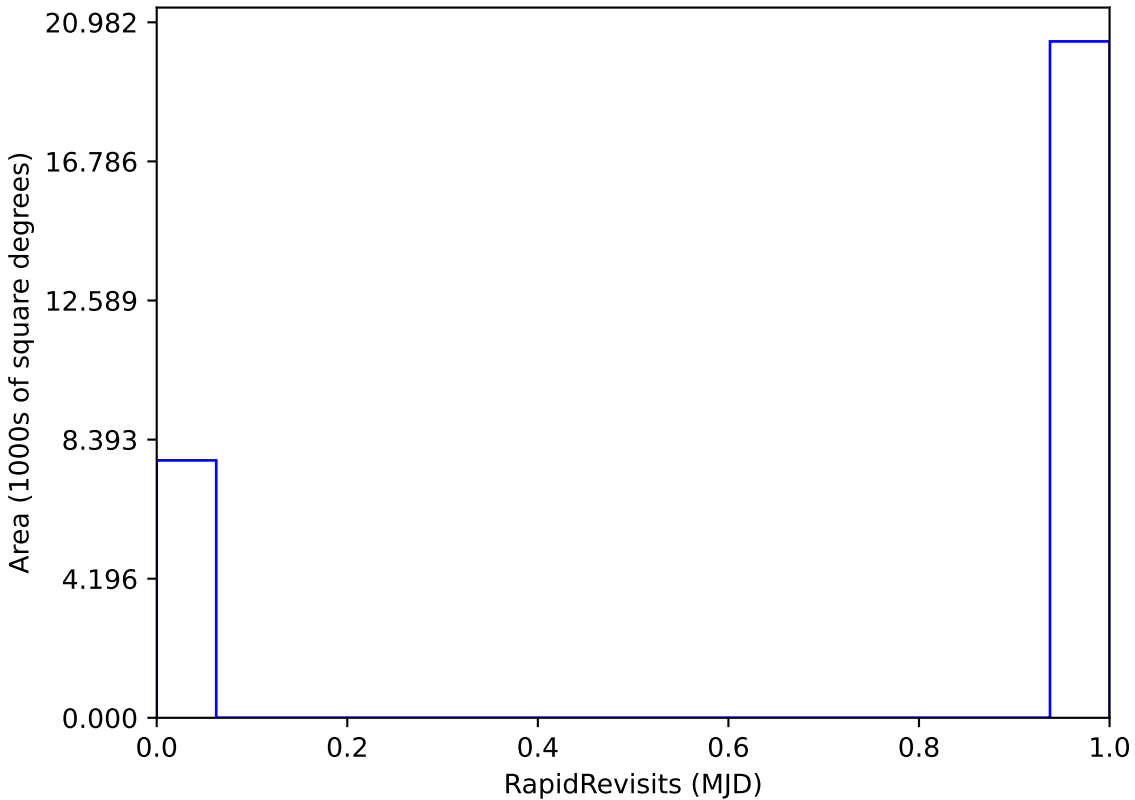
too_elab_2yr_r128_d2_ugrizy_v3.4_10yrs : RapidRevisits
