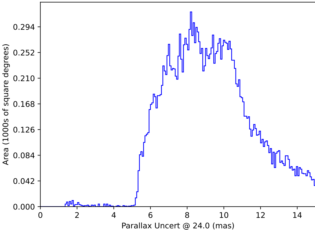
too_elab_2yr_r128_d2_ugrizy_v3.4_10yrs : Parallax Uncert @ 24.0
