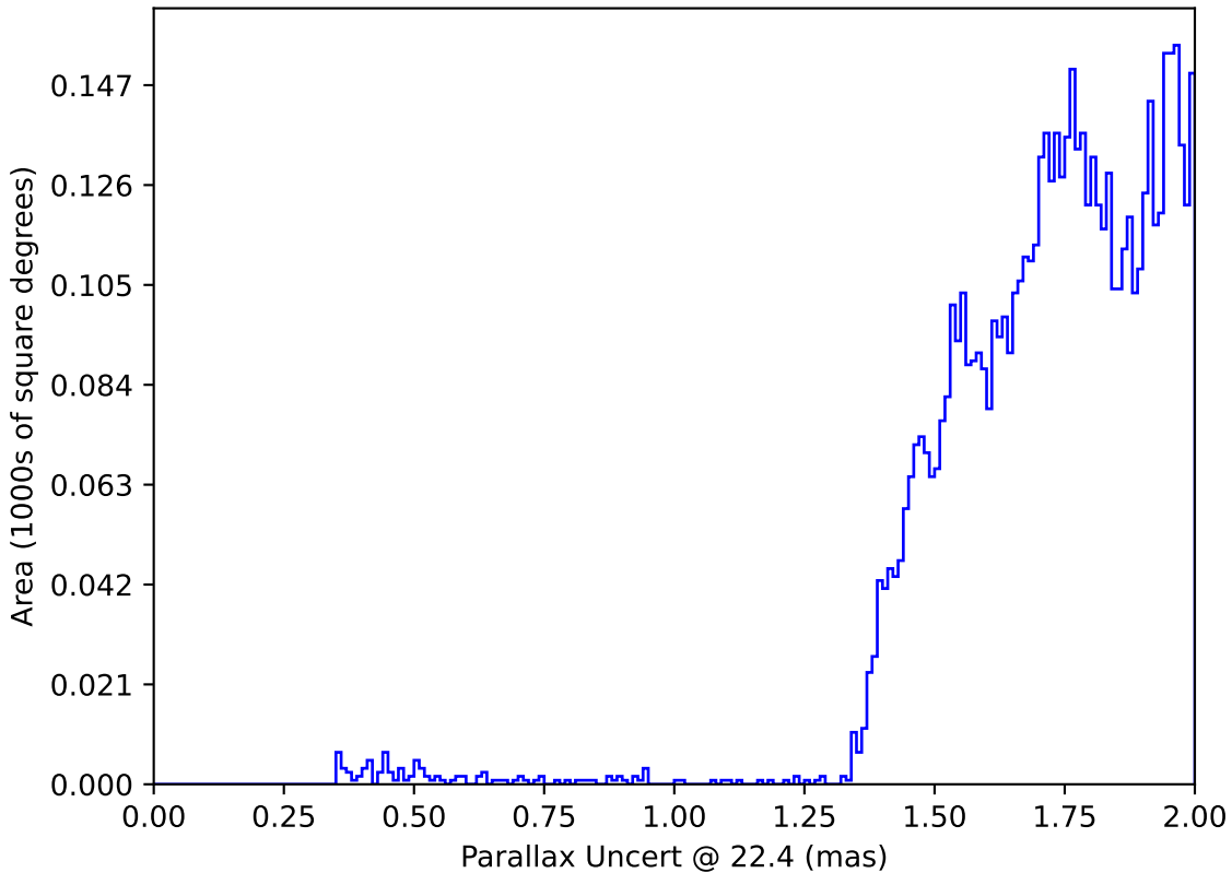
too_elab_2yr_r128_d2_ugrizy_v3.4_10yrs : Parallax Uncert @ 22.4
