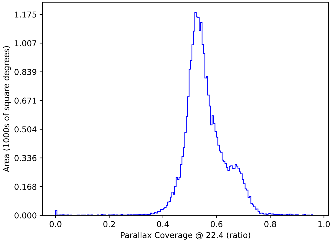
too_elab_2yr_r128_d2_ugrizy_v3.4_10yrs : Parallax Coverage @ 22.4
