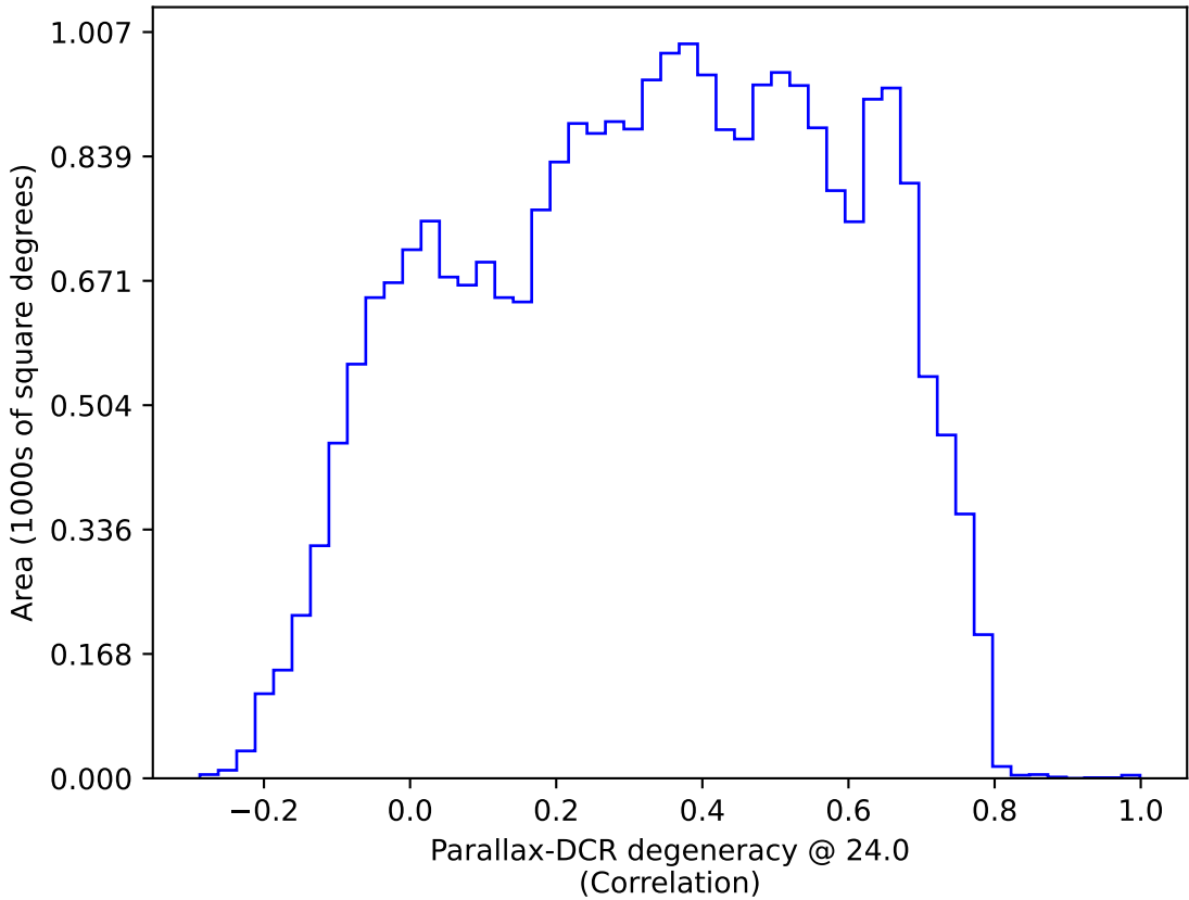
too_elab_2yr_r128_d2_ugrizy_v3.4_10yrs : Parallax-DCR degeneracy @ 24.0
