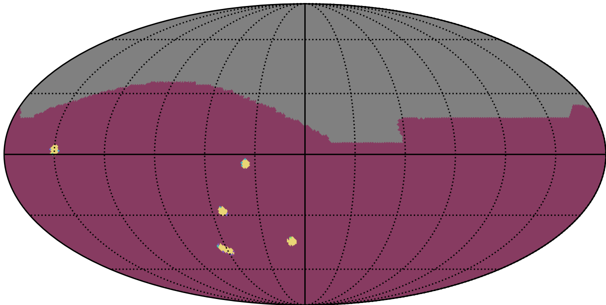
too_elab_2yr_r128_d2_ugrizy_v3.4_10yrs : NumberOfQuickRevisits
