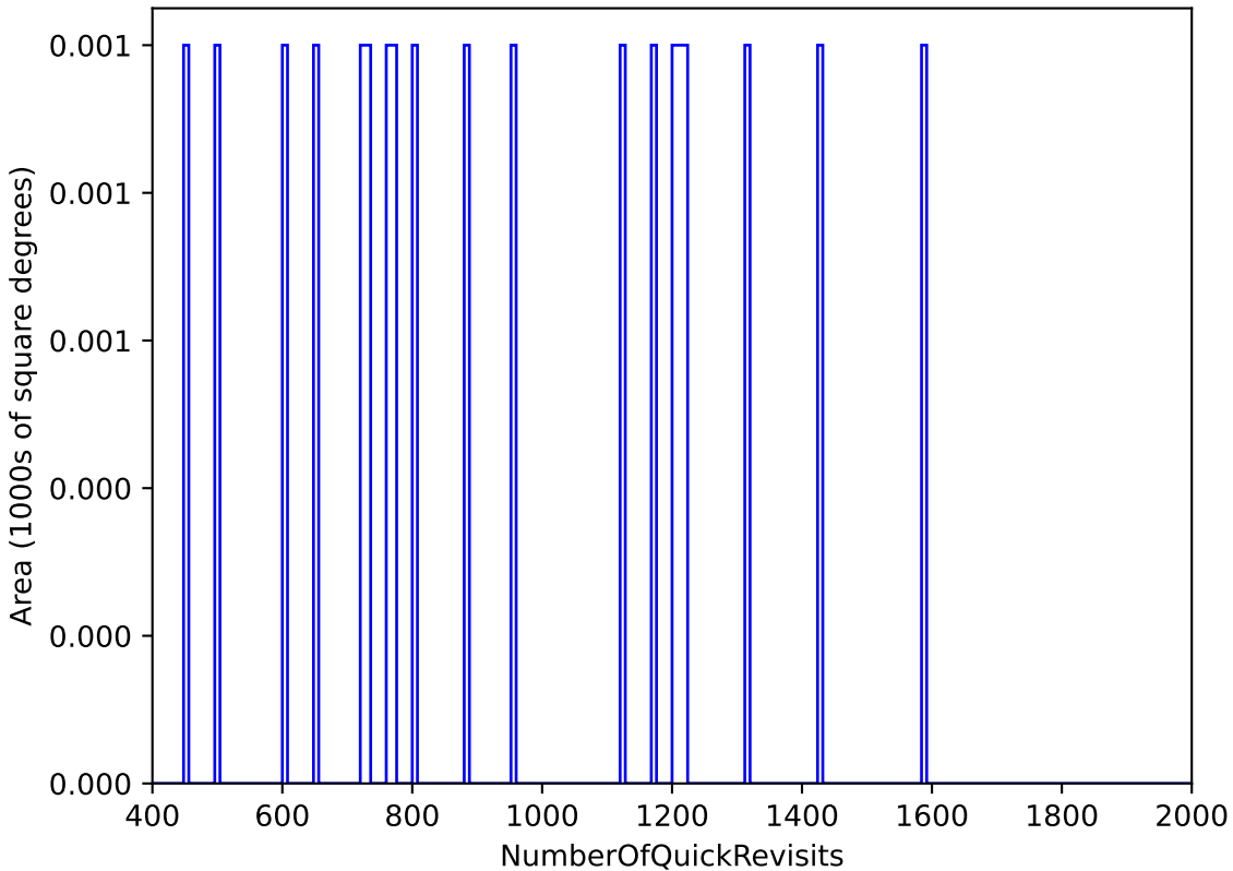
too_elab_2yr_r128_d2_ugrizy_v3.4_10yrs : NumberOfQuickRevisits
