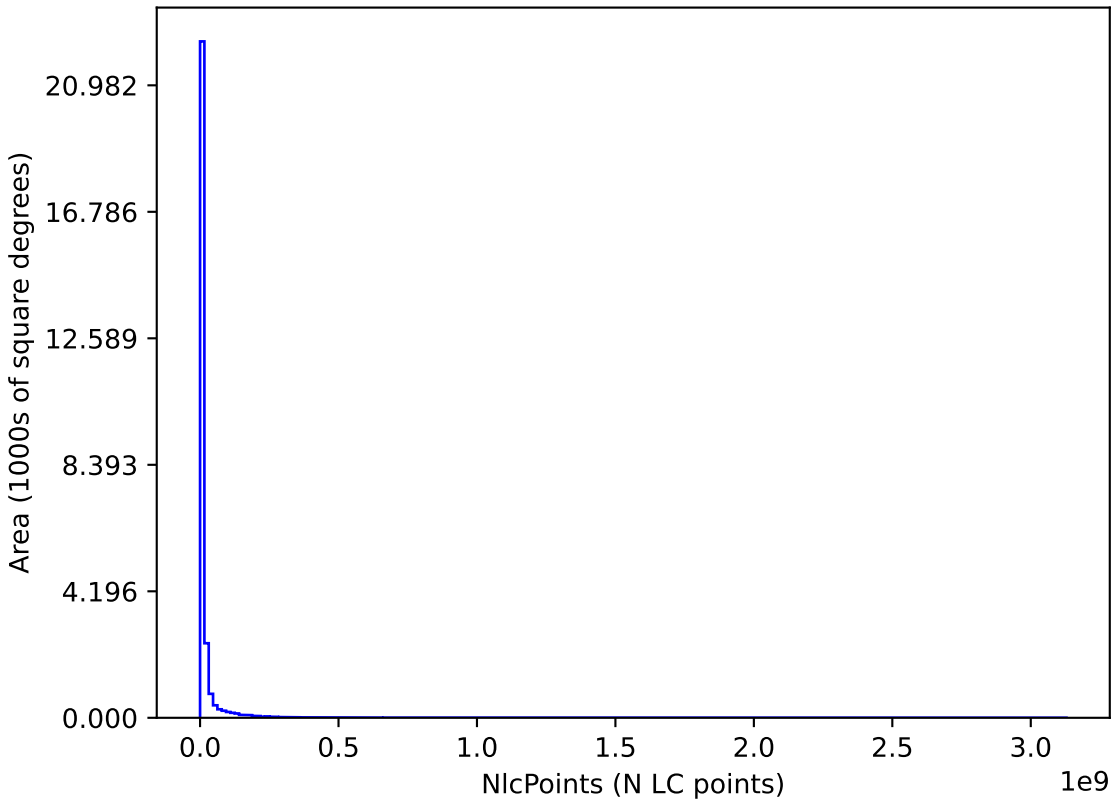
too_elab_2yr_r128_d2_ugrizy_v3.4_10yrs : NlcPoints
