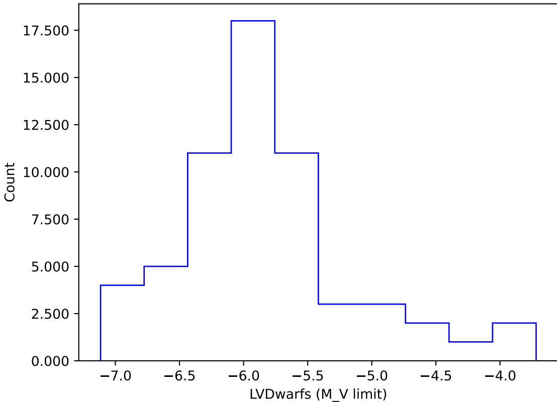
too_elab_2yr_r128_d2_ugrizy_v3.4_10yrs gi: LVDwarfs
