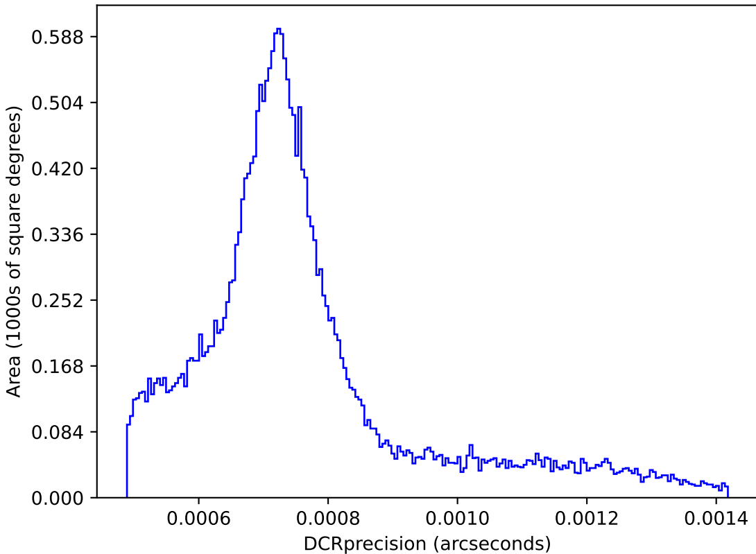
too_elab_2yr_r128_d2_ugrizy_v3.4_10yrs : DCRprecision
