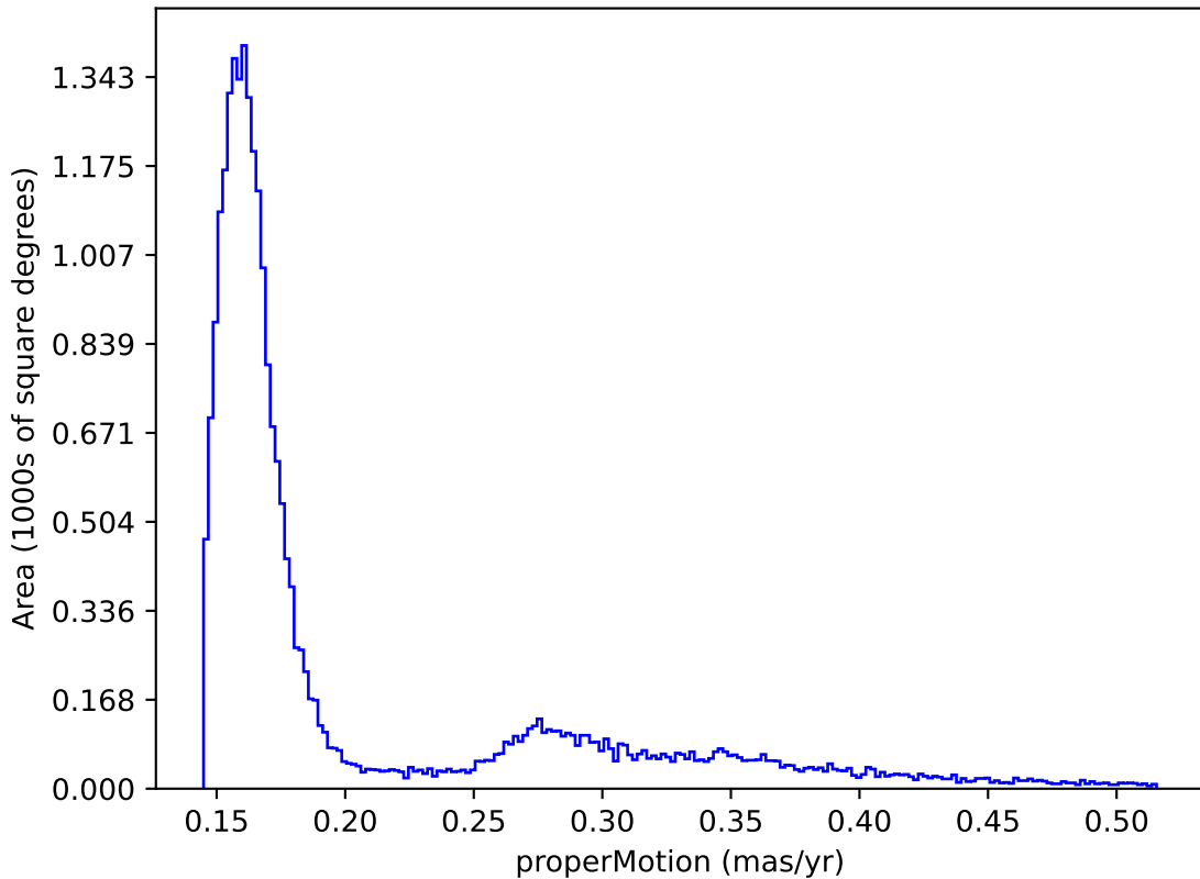
too_elab_2yr_r128_d2_ugrizy_v3.4_10yrs : properMotion
