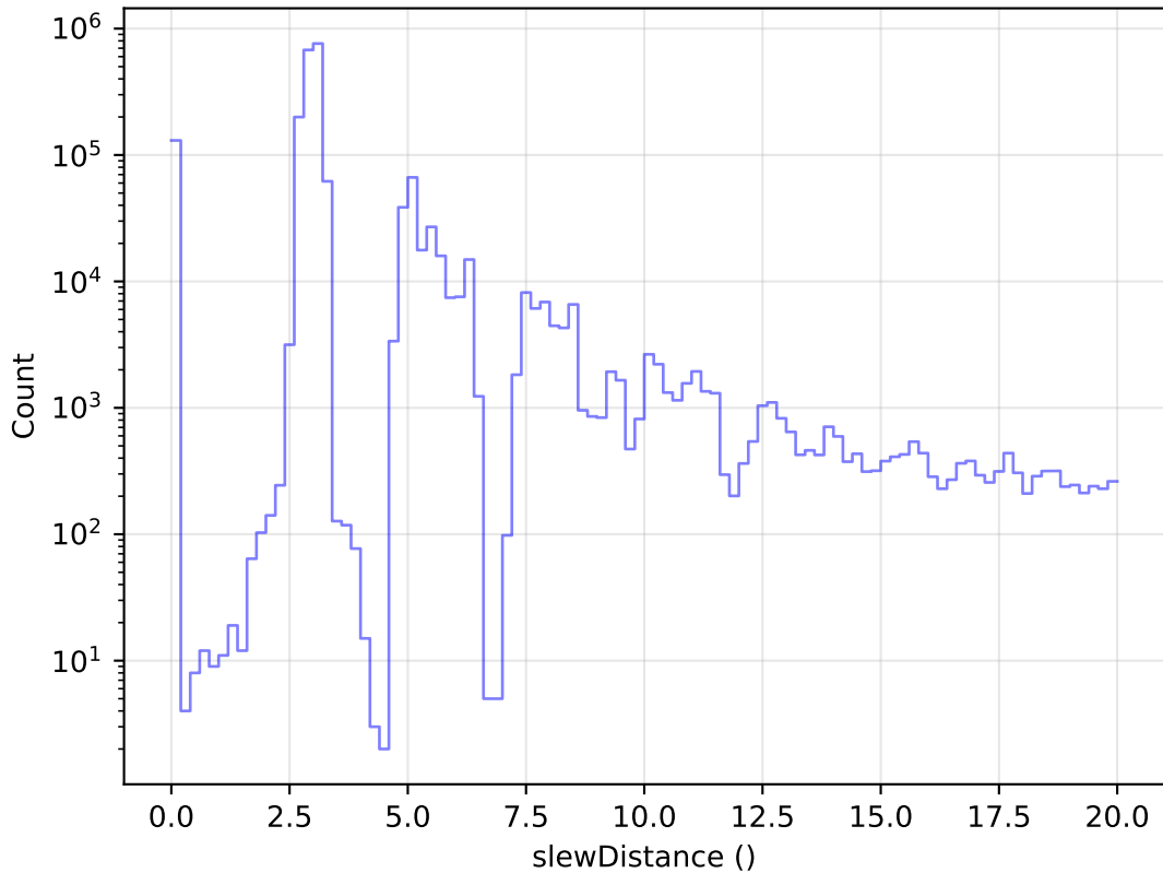
too_elab_2yr_r128_d2_ugrizy_v3.4_10yrs All visits: Zoom Slew Distance Histogram
