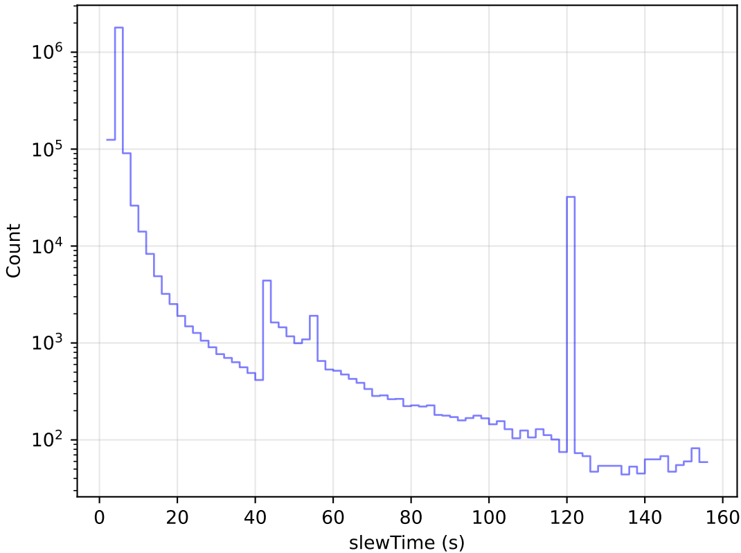
too_elab_2yr_r128_d2_ugrizy_v3.4_10yrs All visits: Slew Time Histogram
