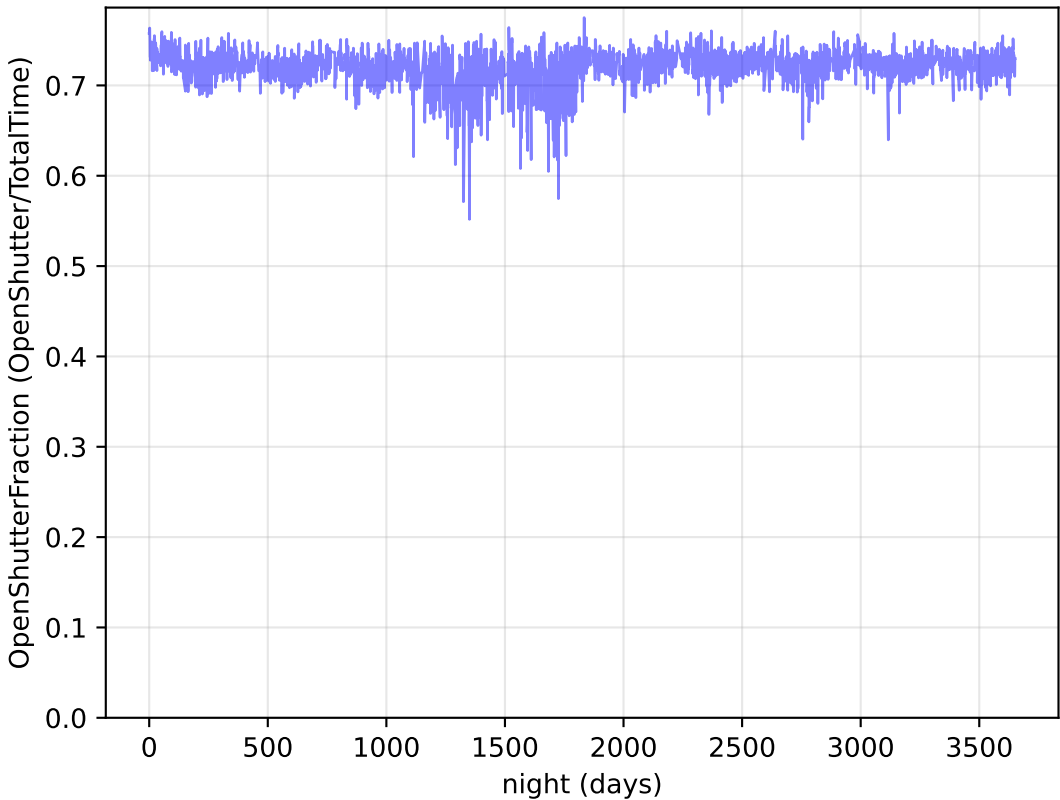
too_elab_2yr_r128_d2_ugrizy_v3.4_10yrs : OpenShutterFraction
