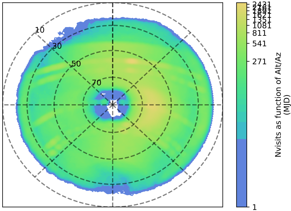
too_elab_2yr_r128_d2_ugrizy_v3.4_10yrs z: Nvisits as function of Alt/Az
