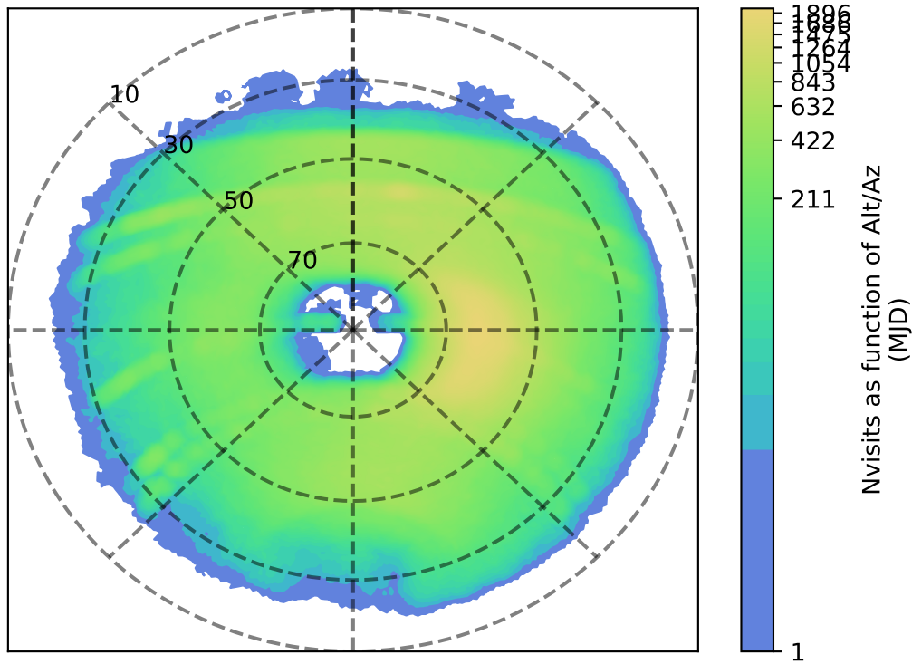
too_elab_2yr_r128_d2_ugrizy_v3.4_10yrs y: Nvisits as function of Alt/Az
