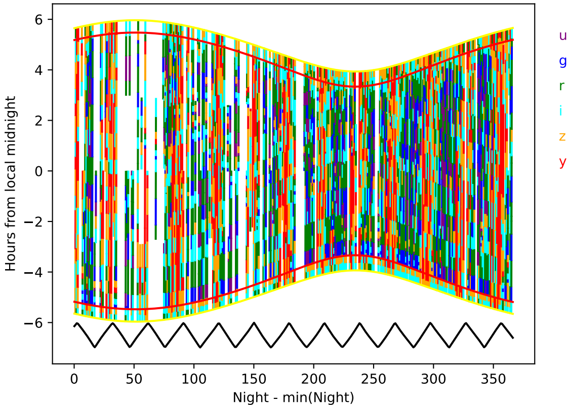
too_elab_2yr_r128_d2_ugrizy_v3.4_10yrs year 9-10: Hourglass
