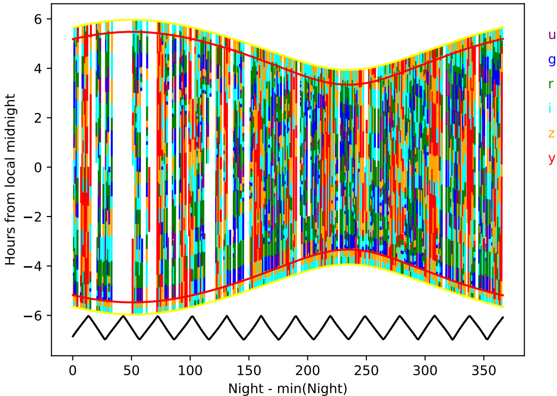
too_elab_2yr_r128_d2_ugrizy_v3.4_10yrs year 8-9: Hourglass
