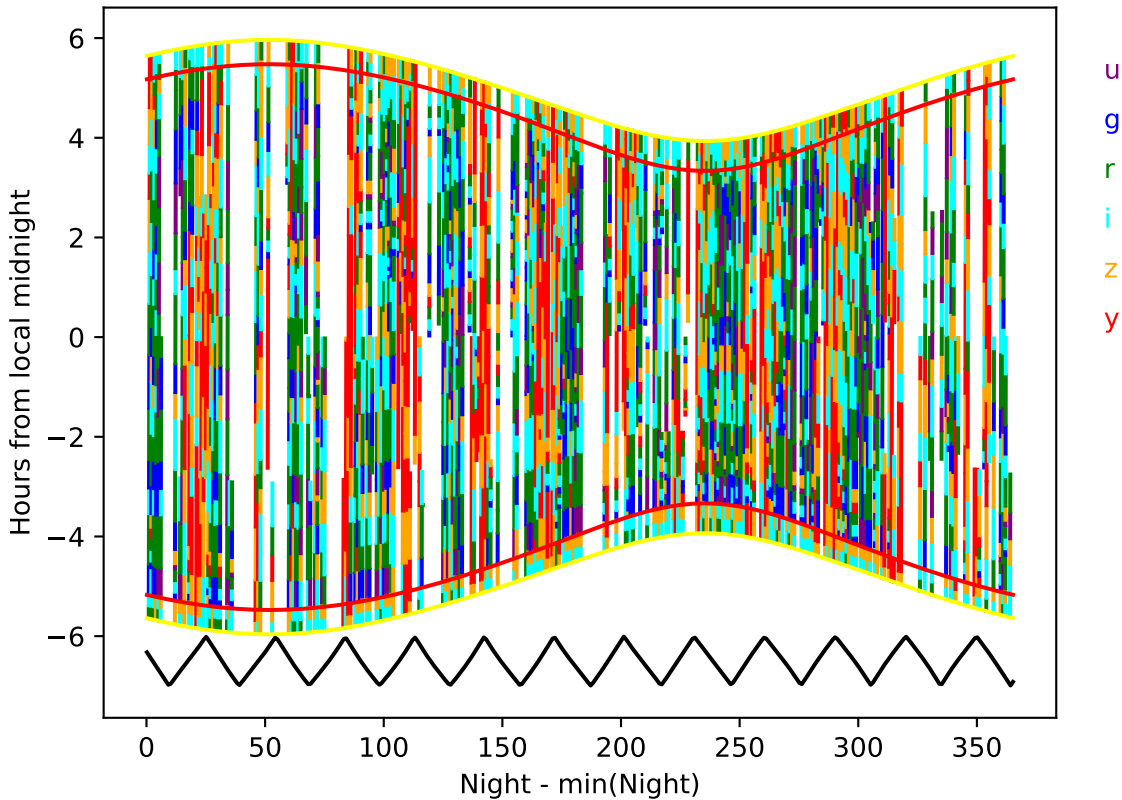
too_elab_2yr_r128_d2_ugrizy_v3.4_10yrs year 7-8: Hourglass
