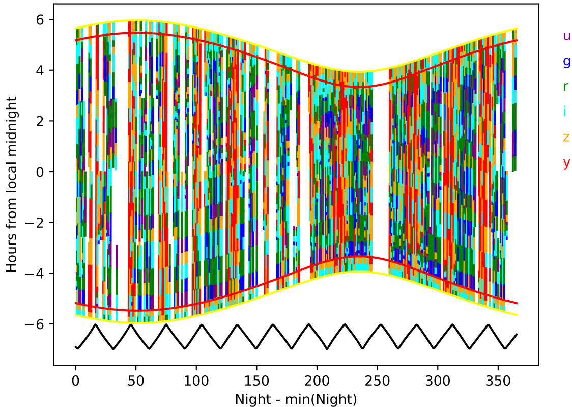
too_elab_2yr_r128_d2_ugrizy_v3.4_10yrs year 5-6: Hourglass
