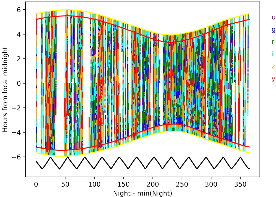
too_elab_2yr_r128_d2_ugrizy_v3.4_10yrs year 4-5: Hourglass
