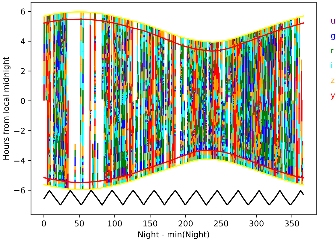
too_elab_2yr_r128_d2_ugrizy_v3.4_10yrs year 3-4: Hourglass
