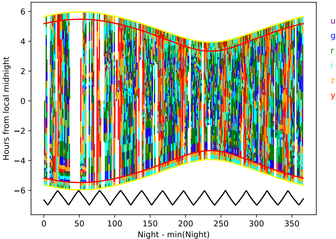
too_elab_2yr_r128_d2_ugrizy_v3.4_10yrs year 2-3: Hourglass
