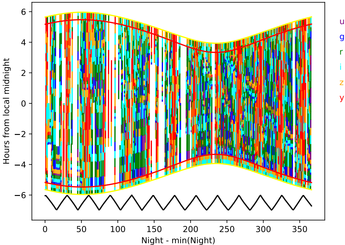
too_elab_2yr_r128_d2_ugrizy_v3.4_10yrs year 1-2: Hourglass
