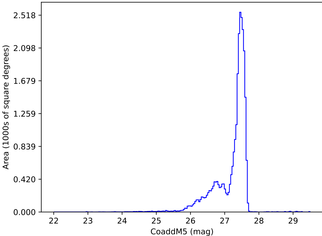
too_elab_2yr_r128_d2_ugrizy_v3.4_10yrs : CoaddM5
