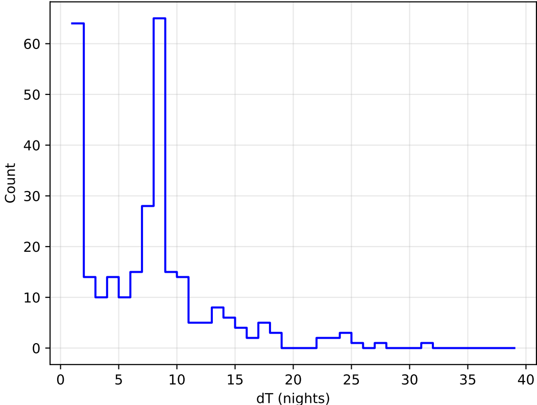
too_elab_2yr_r128_d2_ugrizy_v3.4_10yrs all bands: DD:XMM_LSS Delta Nights Histogram
