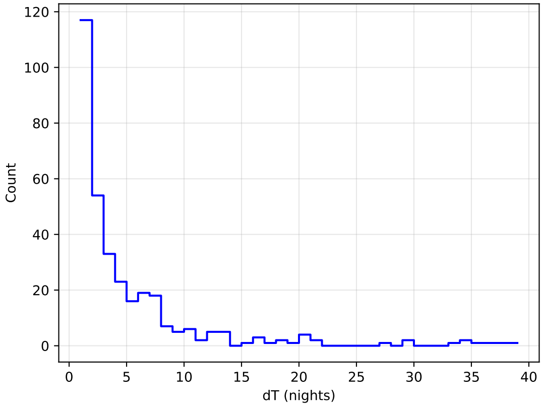
too_elab_2yr_r128_d2_ugrizy_v3.4_10yrs all bands: DD:WFD Delta Nights Histogram
