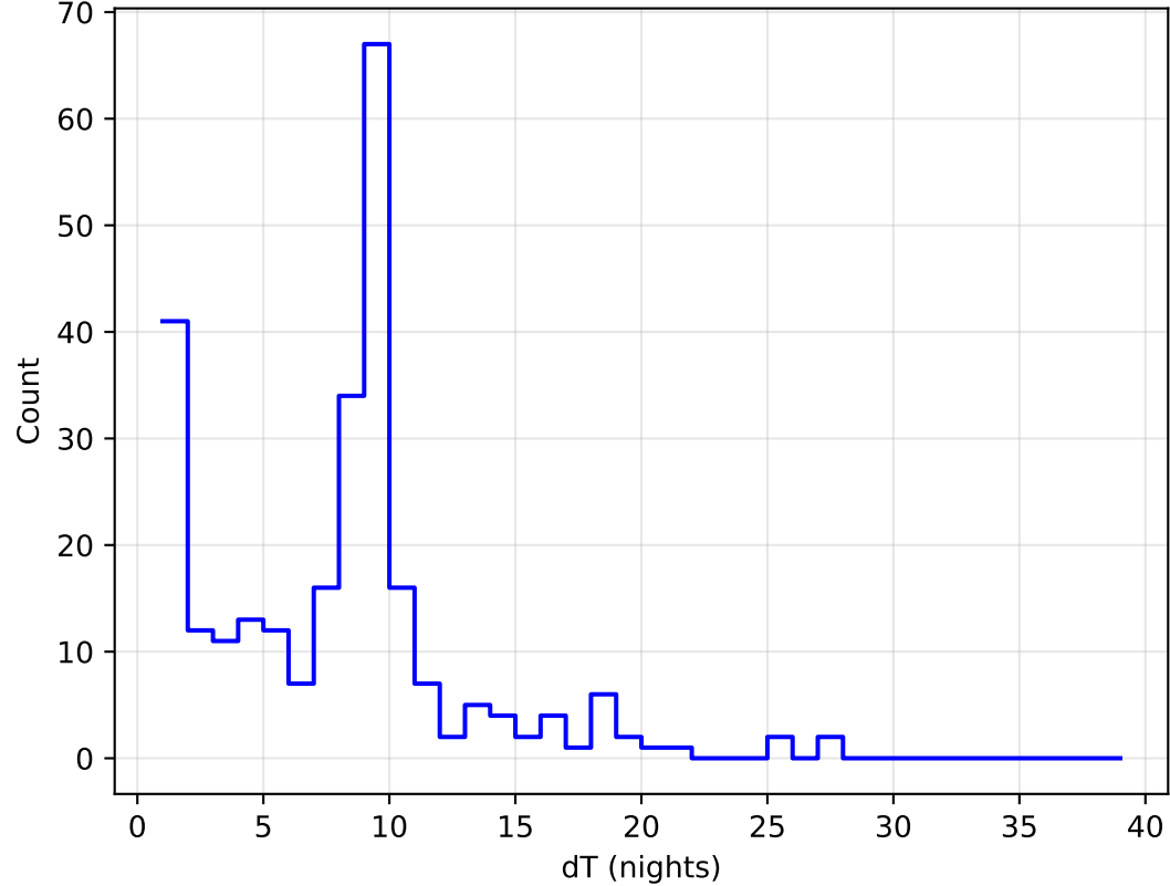
too_elab_2yr_r128_d2_ugrizy_v3.4_10yrs all bands: DD:ELAISS1 Delta Nights Histogram
