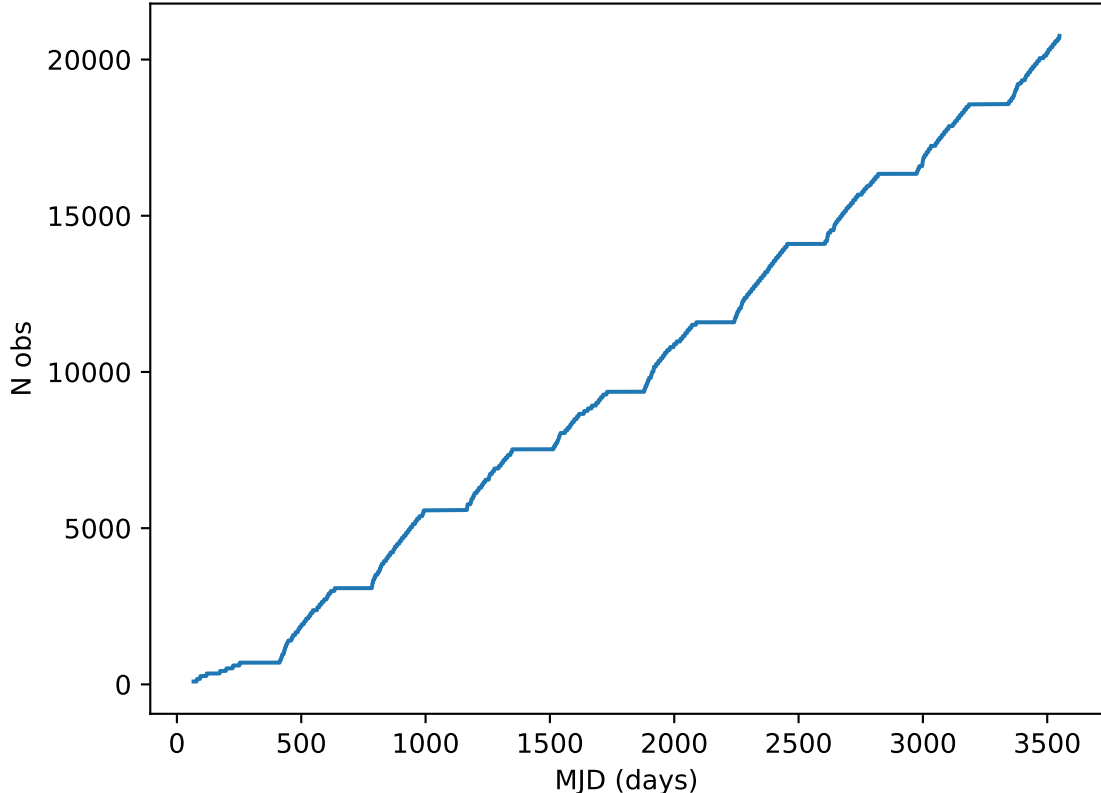
too_elab_2yr_r128_d2_ugrizy_v3.4_10yrs all bands: DD:ELAISS1 Cumulative NVisits
