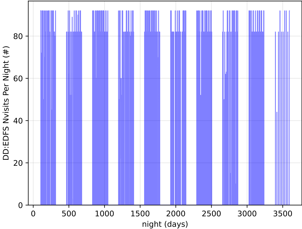
too_elab_2yr_r128_d2_ugrizyv3.4_10yrs all bands: DD:EDFS Nvisits Per Night
