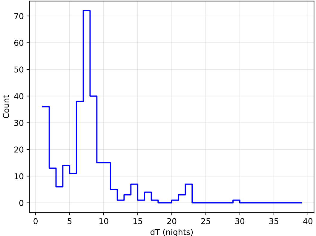
too_elab_2yr_r128_d2_ugrizy_v3.4_10yrs all bands: DD:EDFS Delta Nights Histogram
