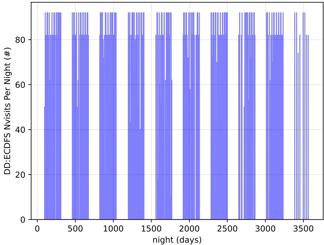
too_elab_2yr_r128_d2_ugrizyv3.4_10yrs all bands: DD:ECDFS Nvisits Per Night
