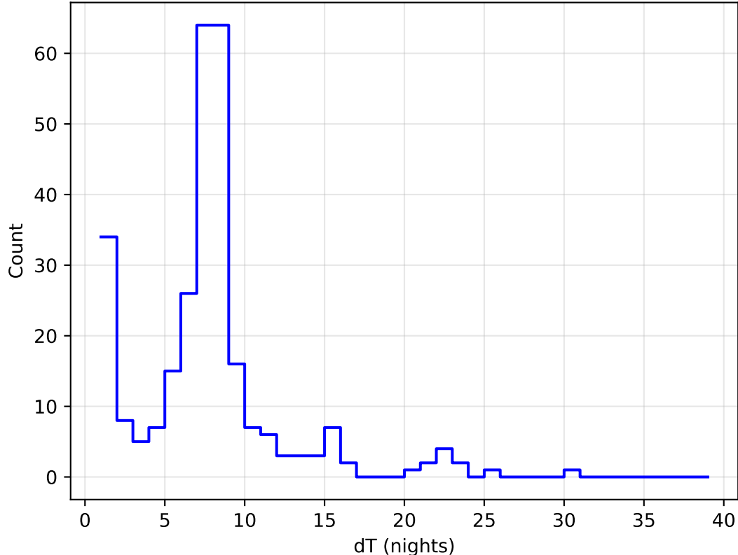
too_elab_2yr_r128_d2_ugrizy_v3.4_10yrs all bands: DD:ECDFS Delta Nights Histogram
