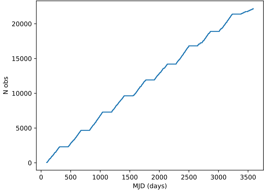
too_elab_2yr_r128_d2_ugrizy_v3.4_10yrs all bands: DD:ECDFS Cumulative NVisits
