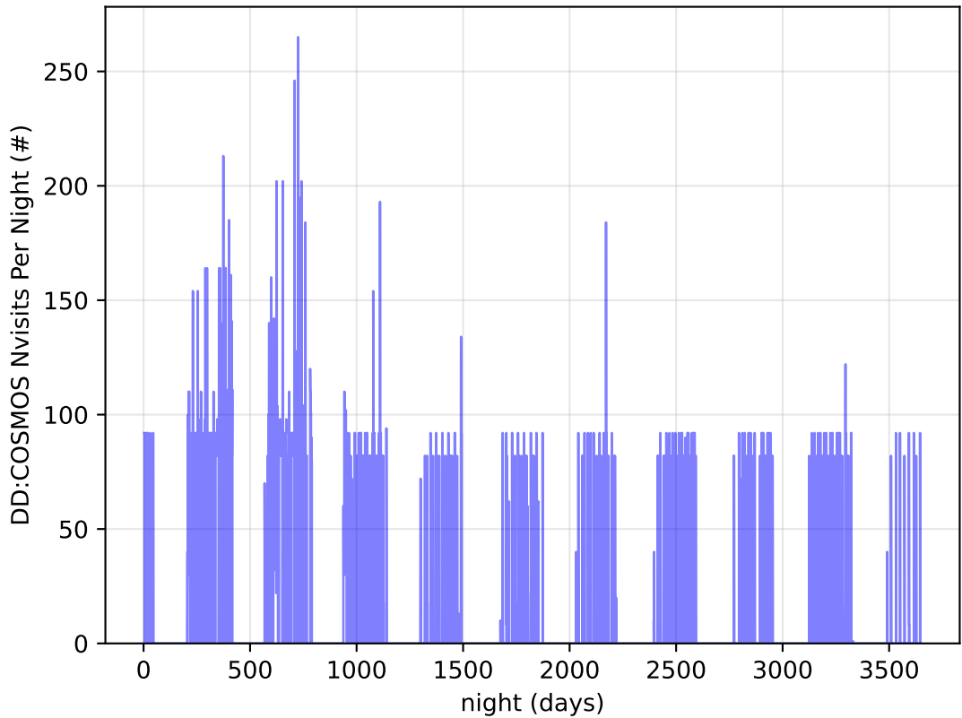
too_elab_2yr_r128_d2_ugrizy_v3.4_10yrs all bands: DD: COSMOS Nvisits Per Night
