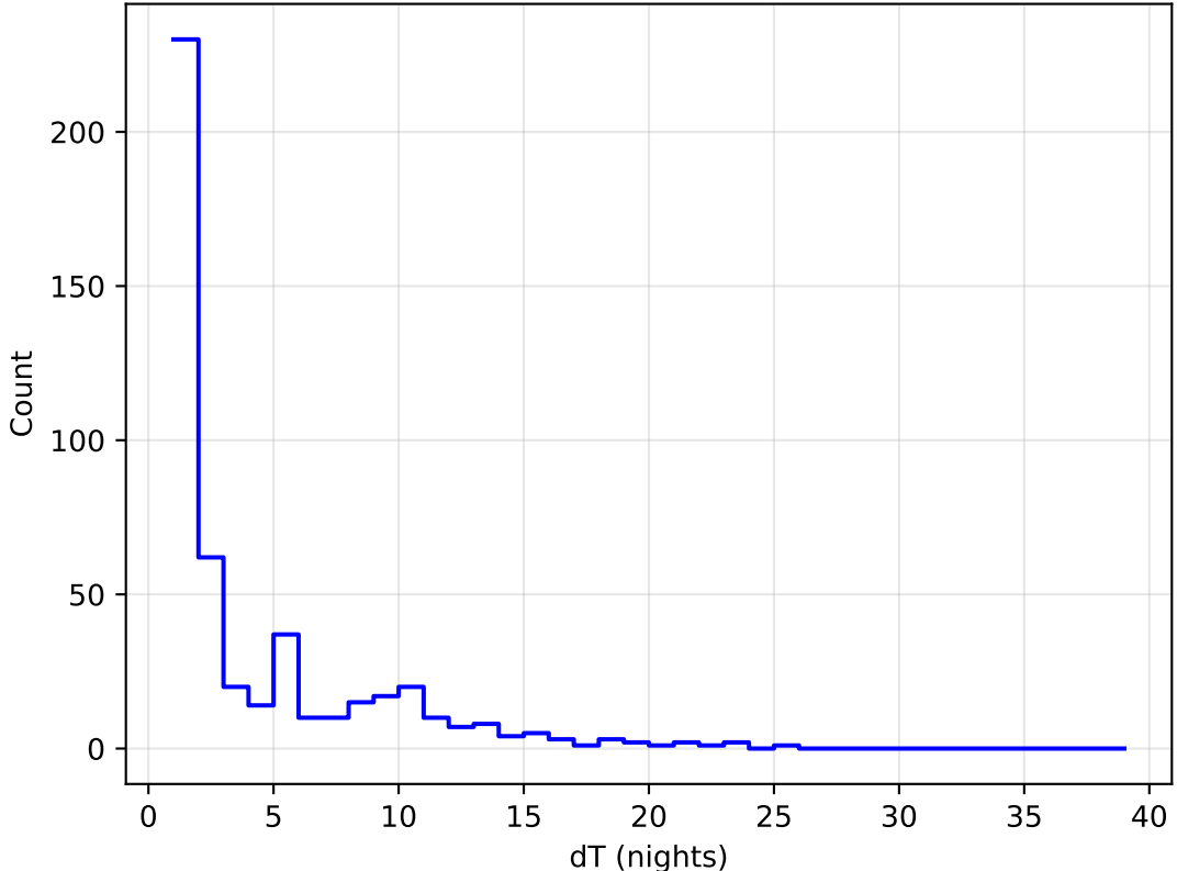
too_elab_2yr_r128_d2_ugrizy_v3.4_10yrs all bands: DD: COSMOS Delta Nights Histogram
