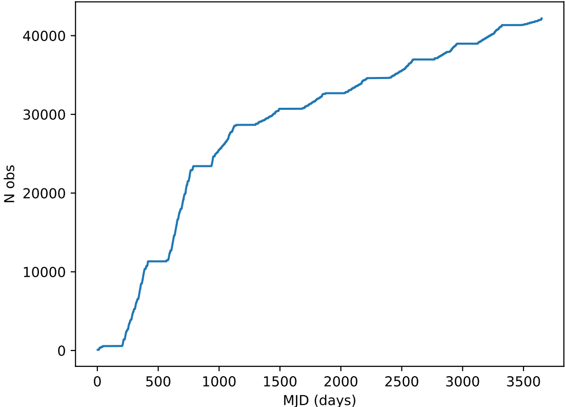
too_elab_2yr_r128_d2_ugrizy_v3.4_10yrs all bands: DD: COSMOS Cumulative NVisits
