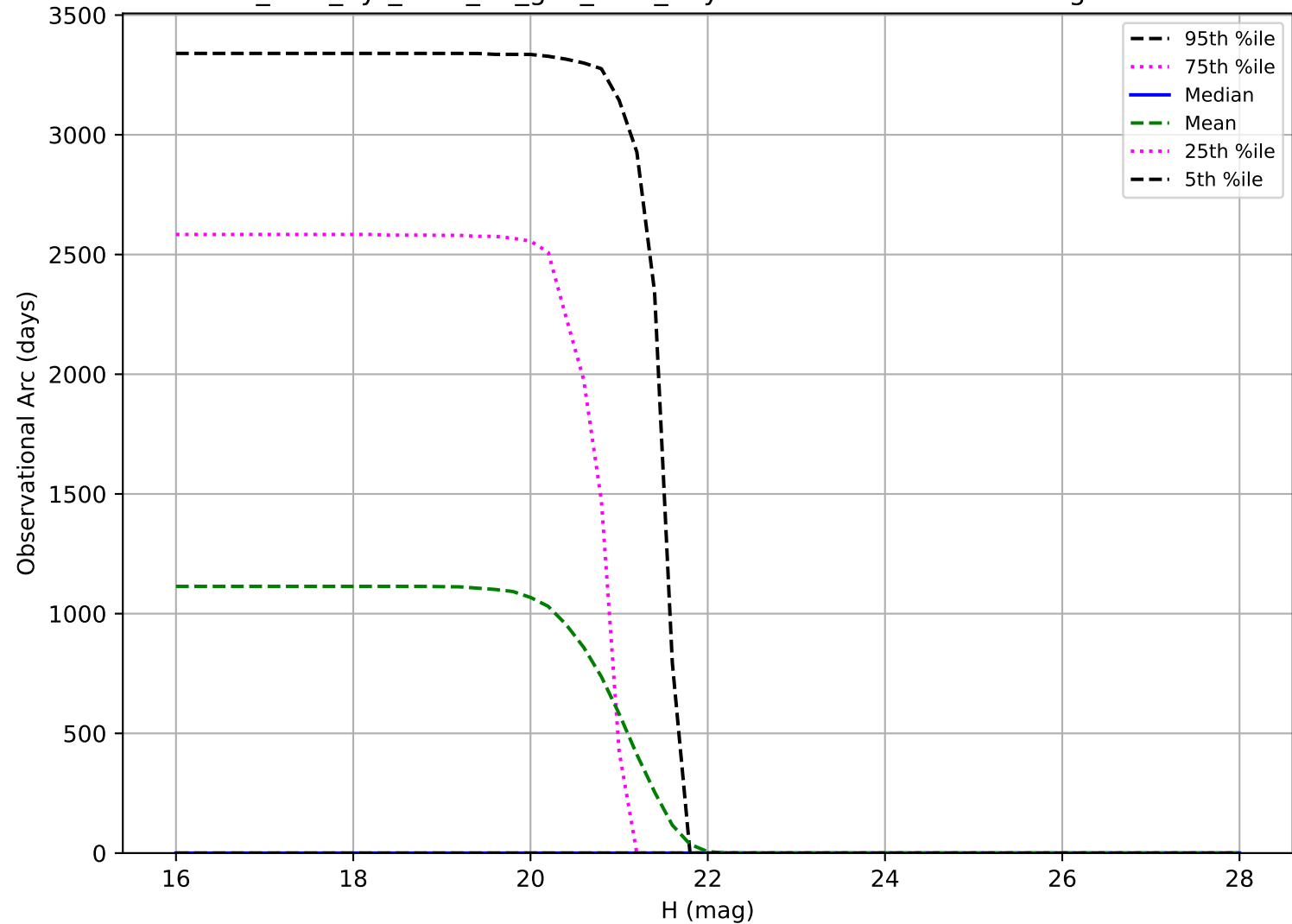
too_elab_2yr_r128_d2_griz_v3.4_10yrs: Observational Arc Length Vatra
