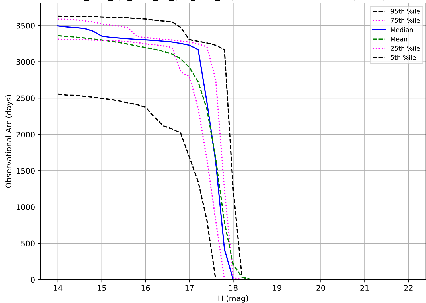
too_elab_2yr_r128_d2_griz_v3.4_10yrs: Observational Arc Length Trojan
