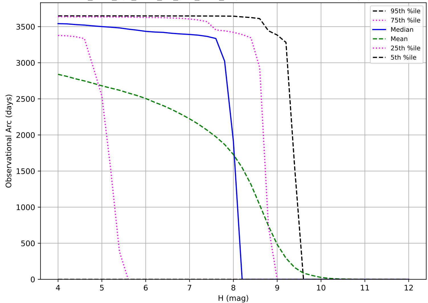
too_elab_2yr_r128_d2_griz_v3.4_10yrs: Observational Arc Length TNO
