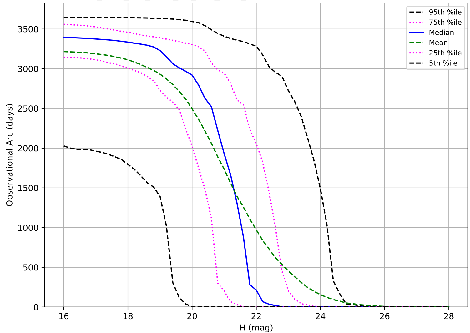
too_elab_2yr_r128_d2_griz_v3.4_10yrs: Observational Arc Length PHA
