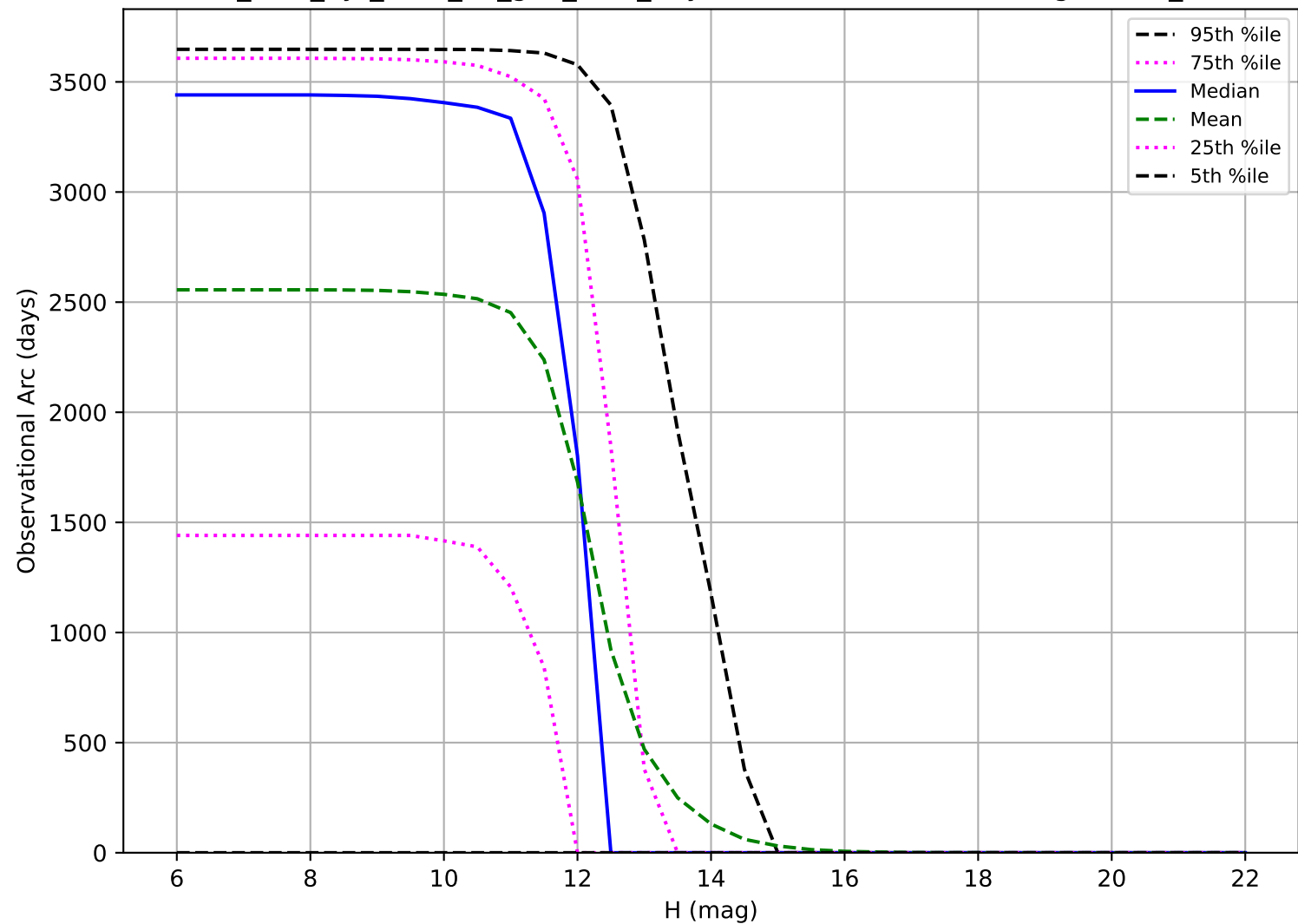
too_elab_2yr_r128_d2_griz_v3.4_10yrs: Observational Arc Length OCC_r20
