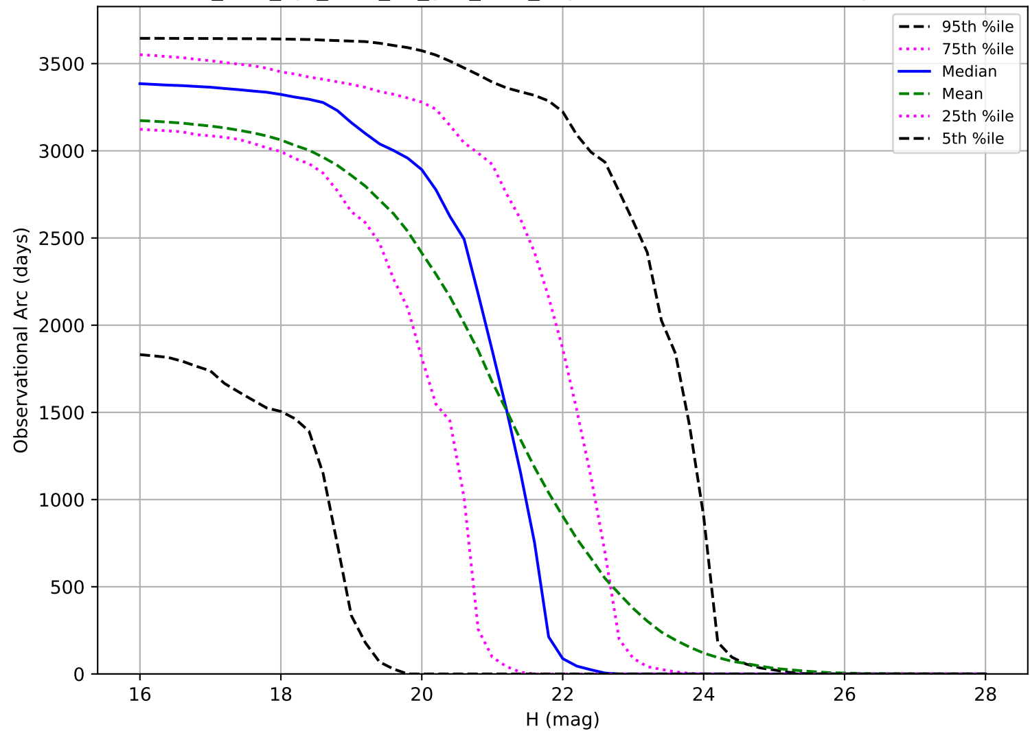
too_elab_2yr_r128_d2_griz_v3.4_10yrs: Observational Arc Length NEO
