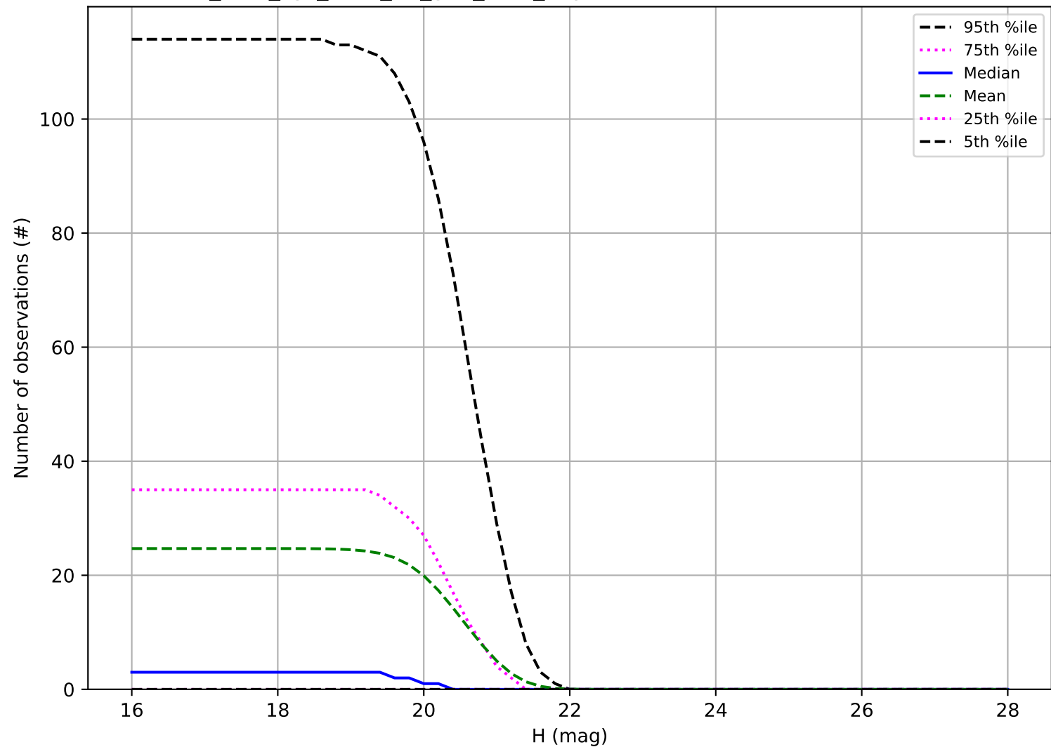
too_elab_2yr_r128_d2_griz_v3.4_10yrs: Number of observations Vatira
