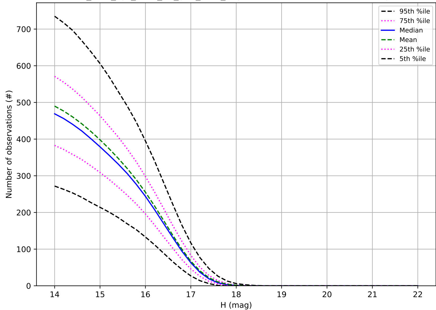
too_elab_2yr_r128_d2_griz_v3.4_10yrs: Number of observations Trojan
