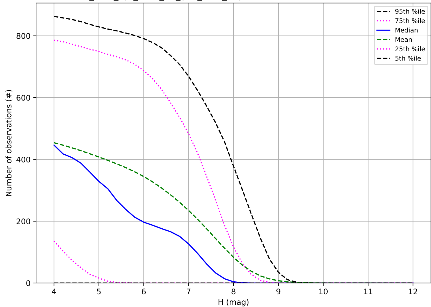
too_elab_2yr_r128_d2_griz_v3.4_10yrs: Number of observations TNO
