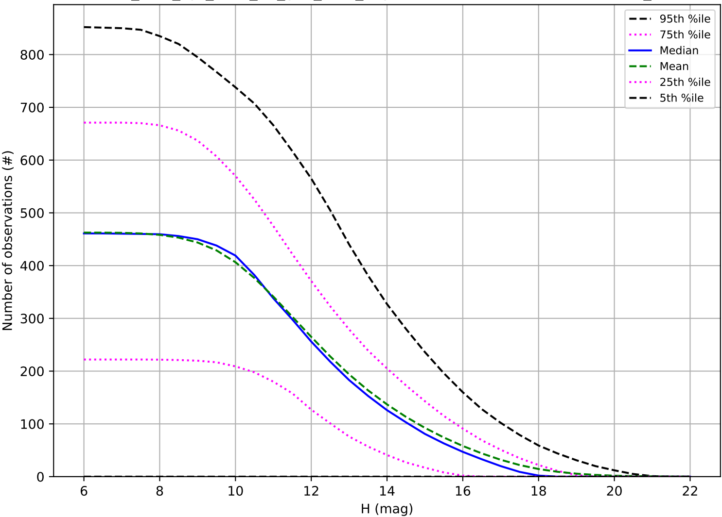
too_elab_2yr_r128_d2_griz_v3.4_10yrs: Number of observations OCC_r5
