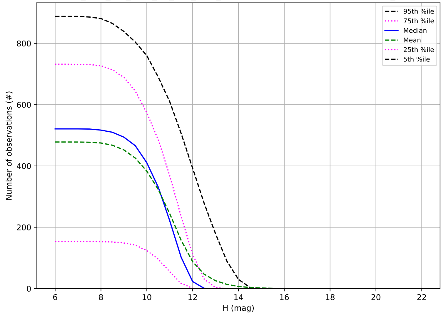
too_elab_2yr_r128_d2_griz_v3.4_10yrs: Number of observations OCC_r20
