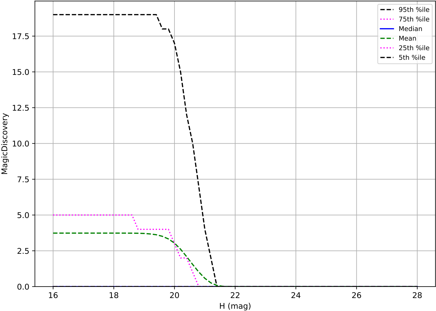
too_elab_2yr_r128_d2_griz_v3.4_10yrs: Vatira 6 detections in 60 nights detection loss
